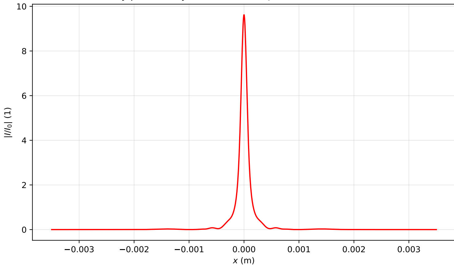
Intensity profile I(x, y = 0, z = 2.149)/I_0 , P_{in}=2.5P_{cr} , artificial time
